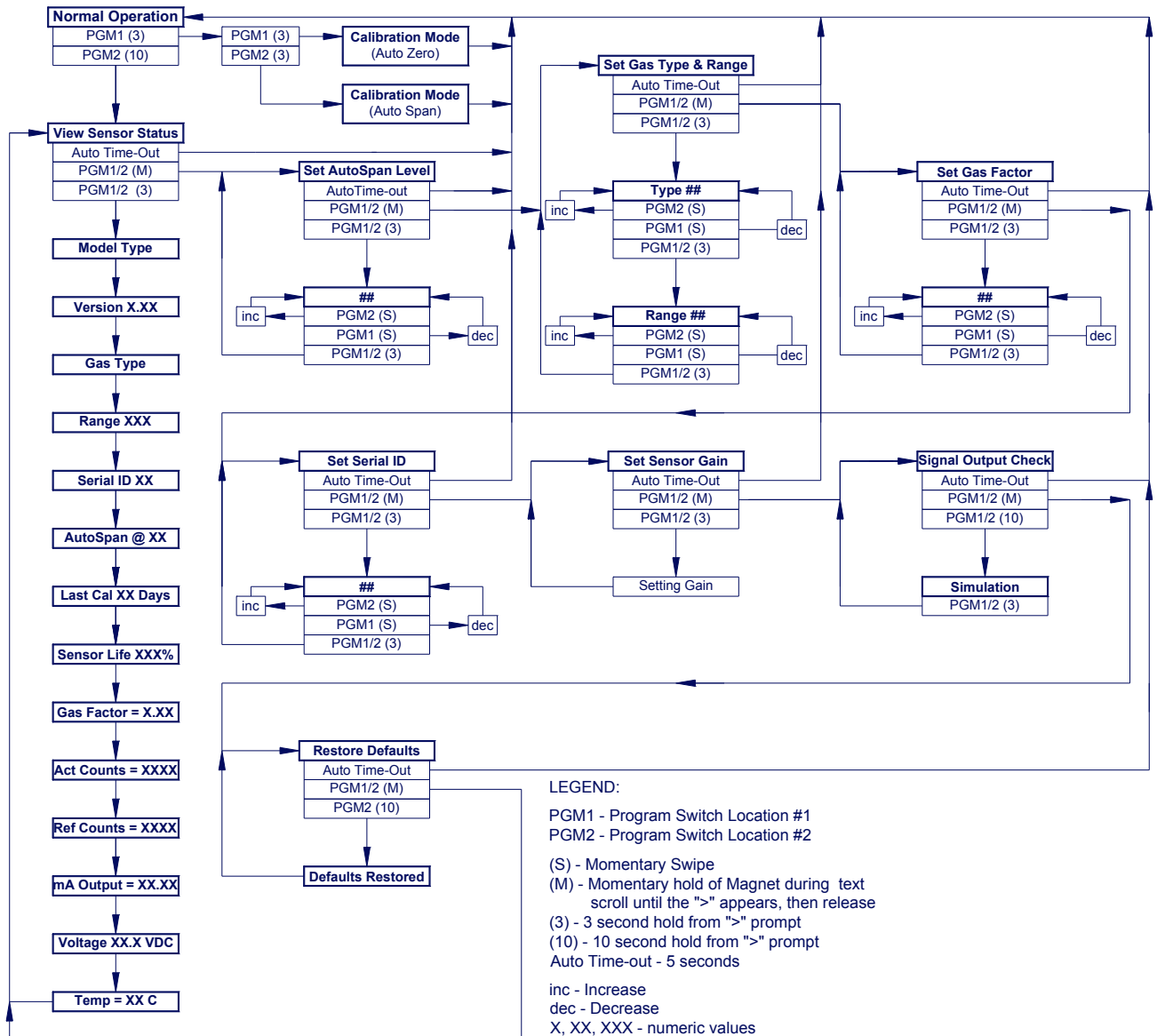
Figure 13 FP-700 Software Flowchart
