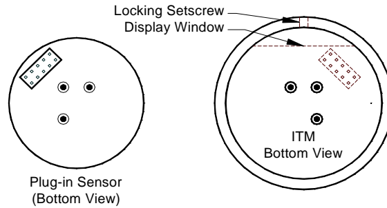
Figure 32 Sensor Cell and ITM Mating
