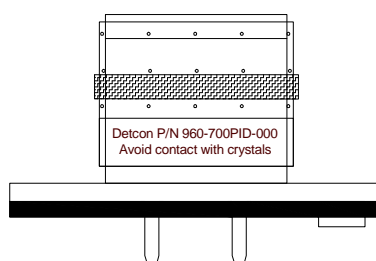
Figure 16 Plug-in sensor with Moisture control packet
