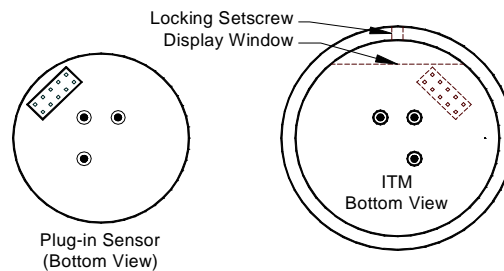
Figure 33 Sensor Cell and ITM Mating
