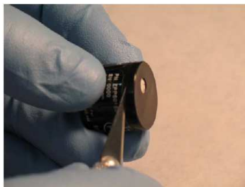
Figure 18 Removal of Filter Cap
