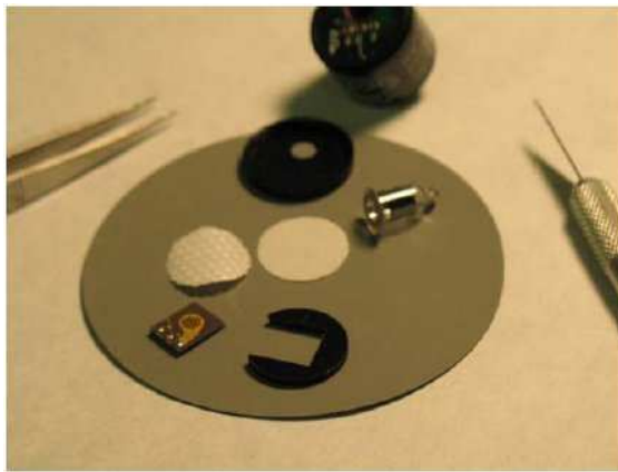
Figure 23 Lamp cleaning
