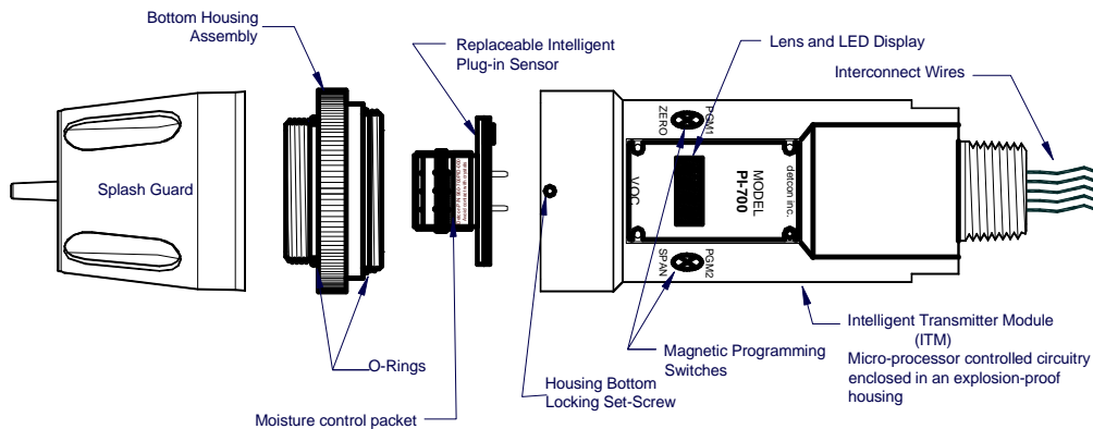
Figure 4 Sensor Assembly Breakaway
