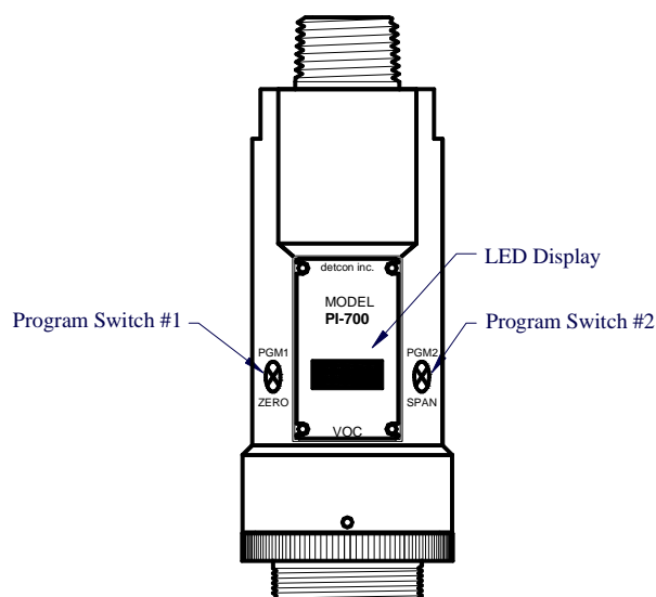
Figure 3 Sensor Assembly Front View
