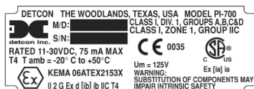
Figure 6 PI-700 ATEX Approval Label
