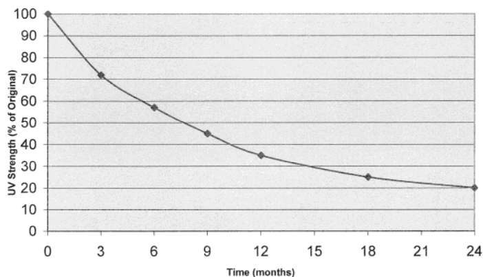
Figure 14 UV Lamp Aging Expectation
