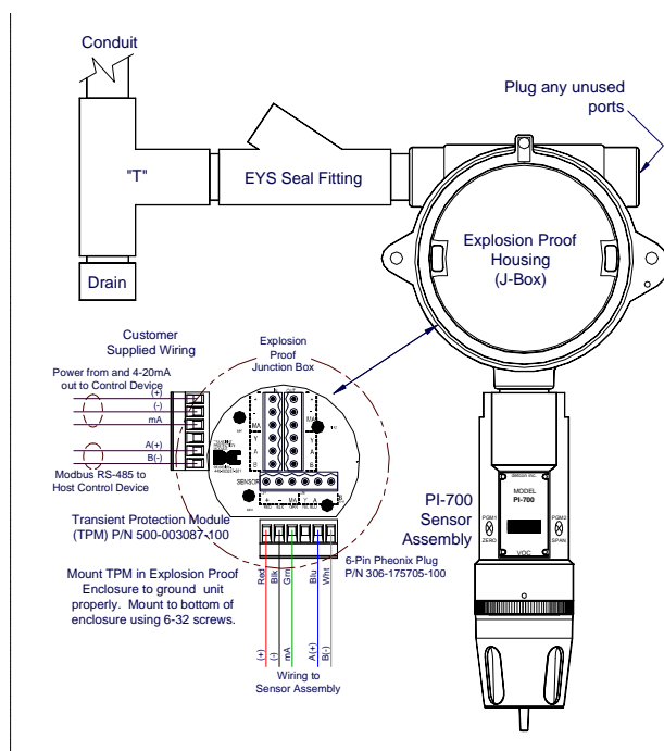
Figure 8 Typical Installation
