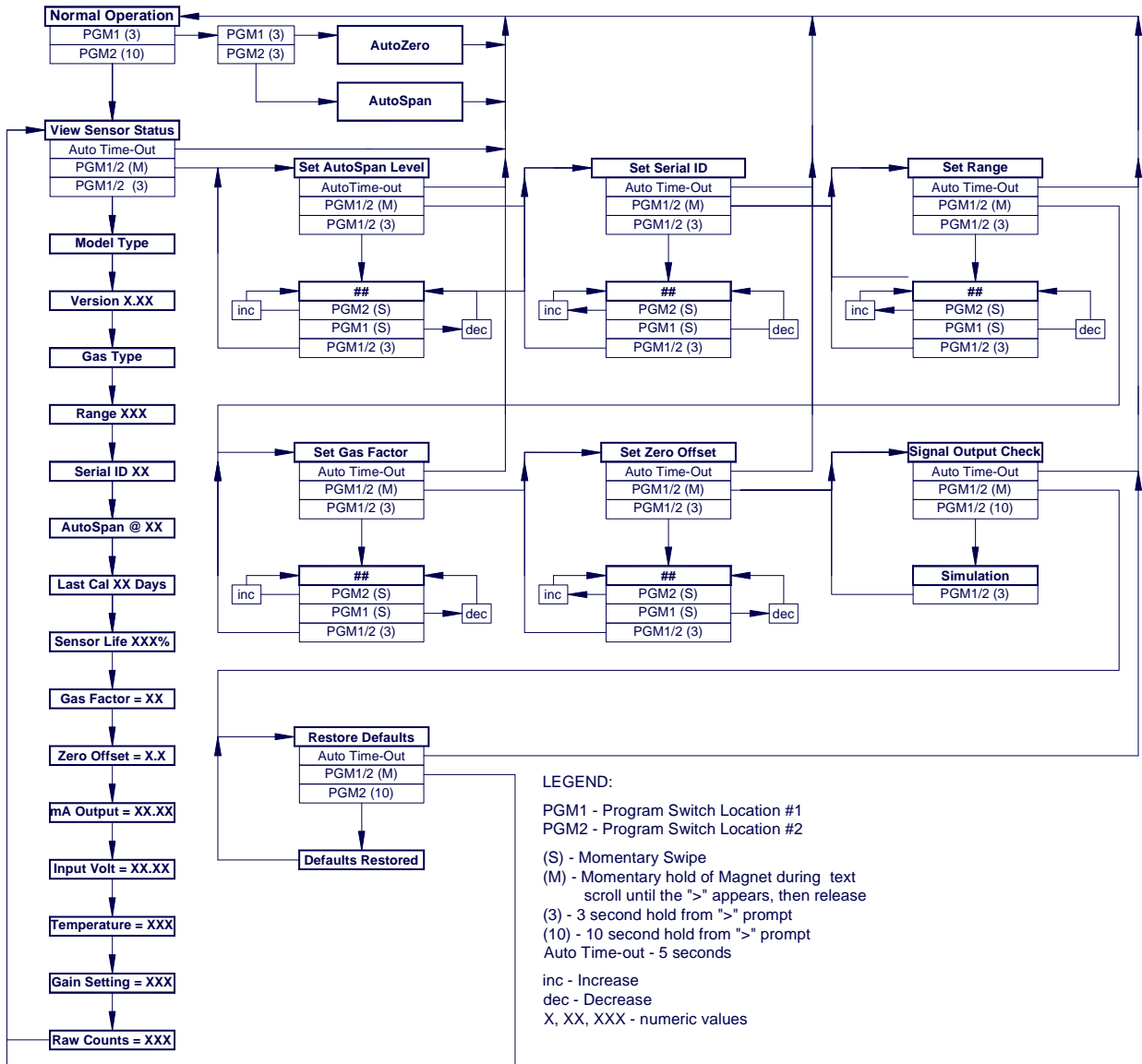
Figure 12 PI-700 Software Flowchart
