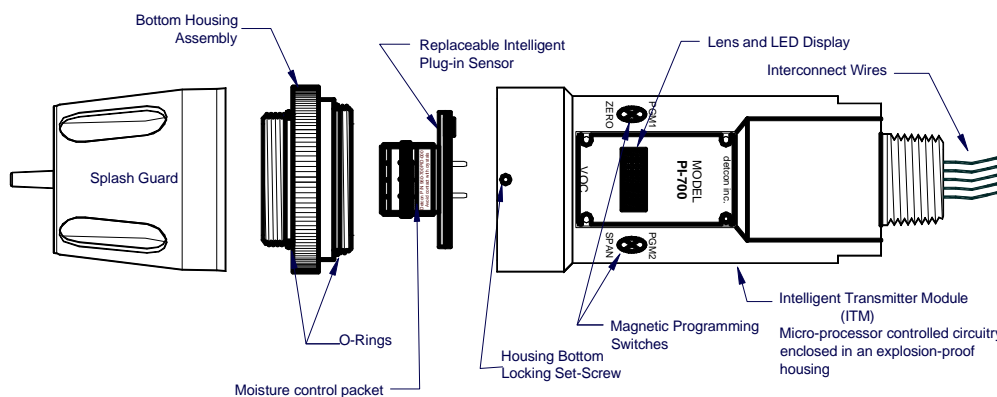
Figure 31 Sensor Assembly
