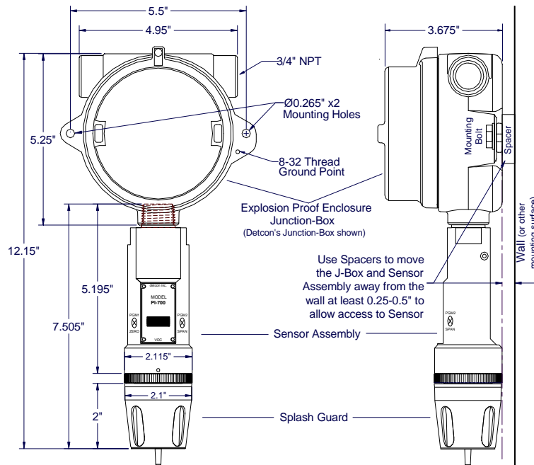
Figure 7 Outline and Mounting Dimensions
