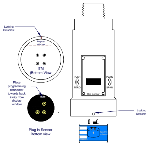
Figure 16 Sensor Cell and ITM Mating
