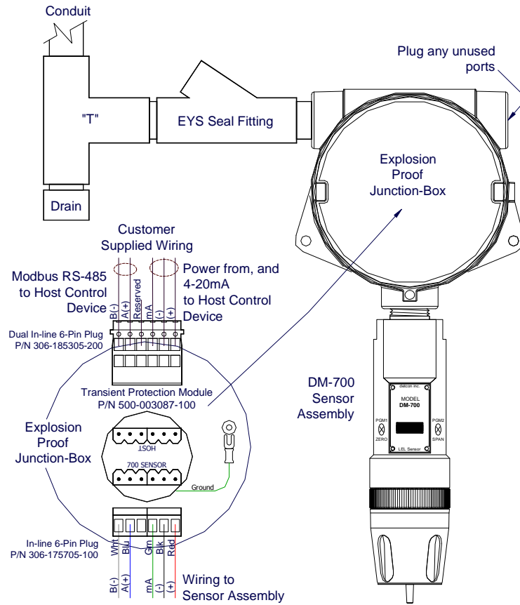
Figure 9 Typical Installation
