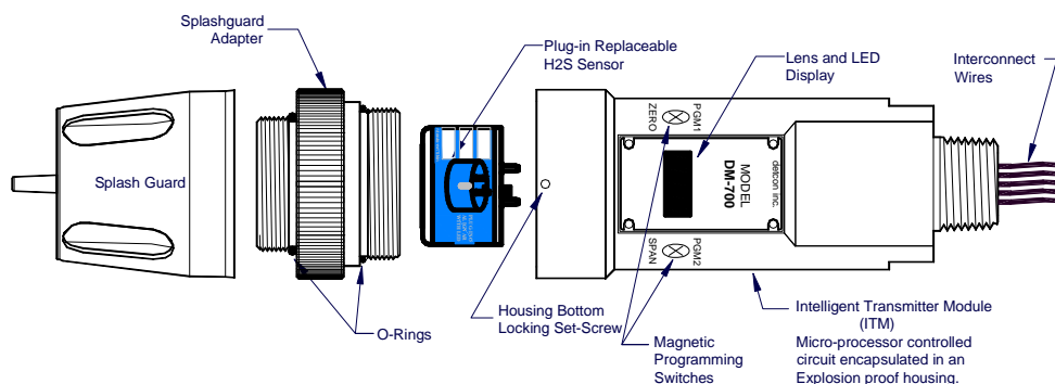
Figure 15 Sensor Assembly
