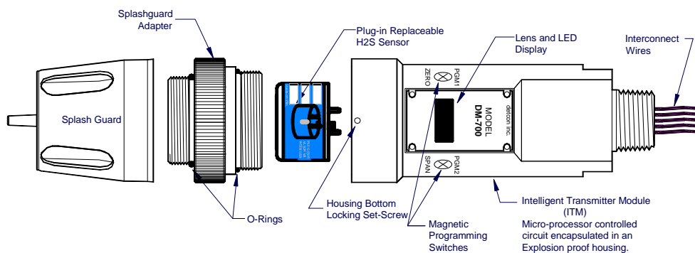
Figure 5 Sensor Assembly Breakaway
