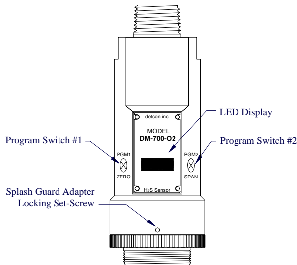
Figure 4 Sensor Assembly Front View
