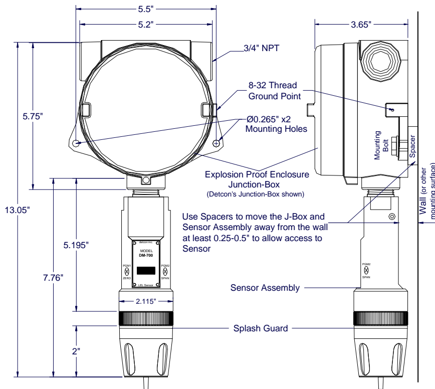
Figure 8 Outline and Mounting Dimensions
