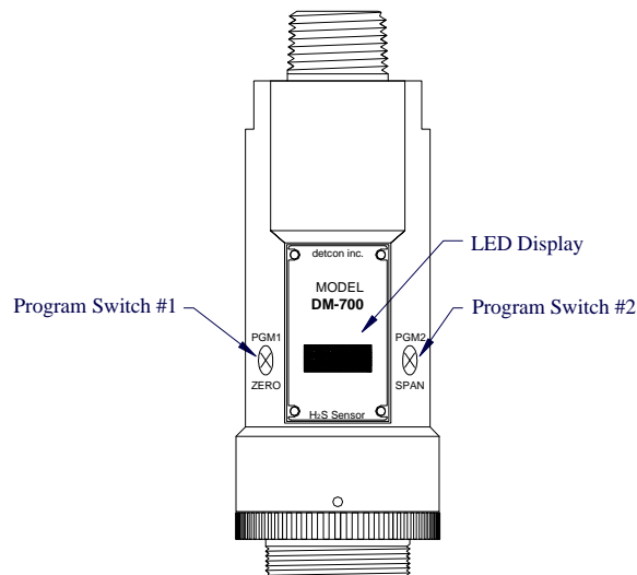
Figure 12 Magnetic Programming Switches
