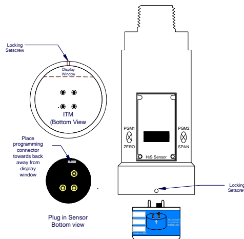
Figure 17 Sensor Cell and ITM Mating
