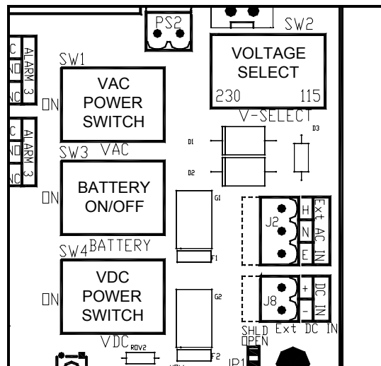
Figure 6 Power Switch Configuration
