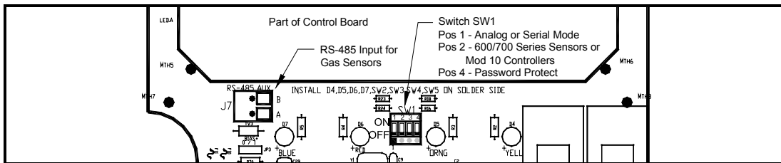
Figure 7 Switch SW1
