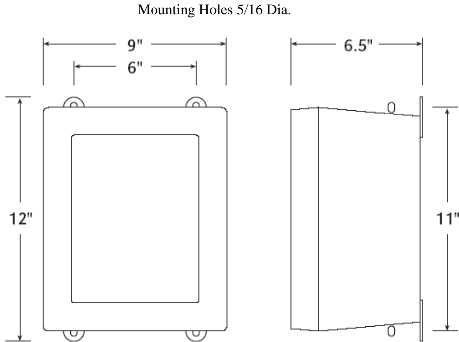
Figure 2 Dimensional View of Enclosures
