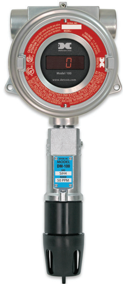
(shown as PN 961-230022-050 in Aluminum j-box with Loop Powered Display)
